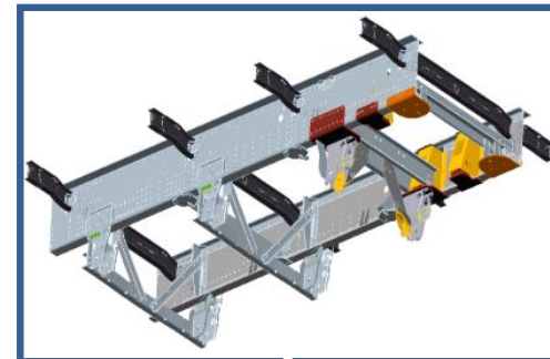
Integration of drive axle
